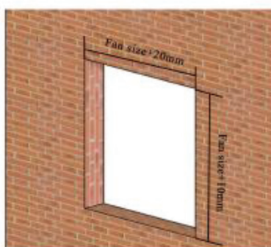
Dimension drawing of reserved hole
